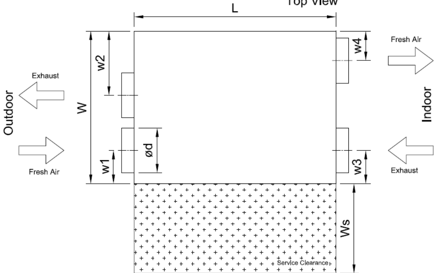
Top View
